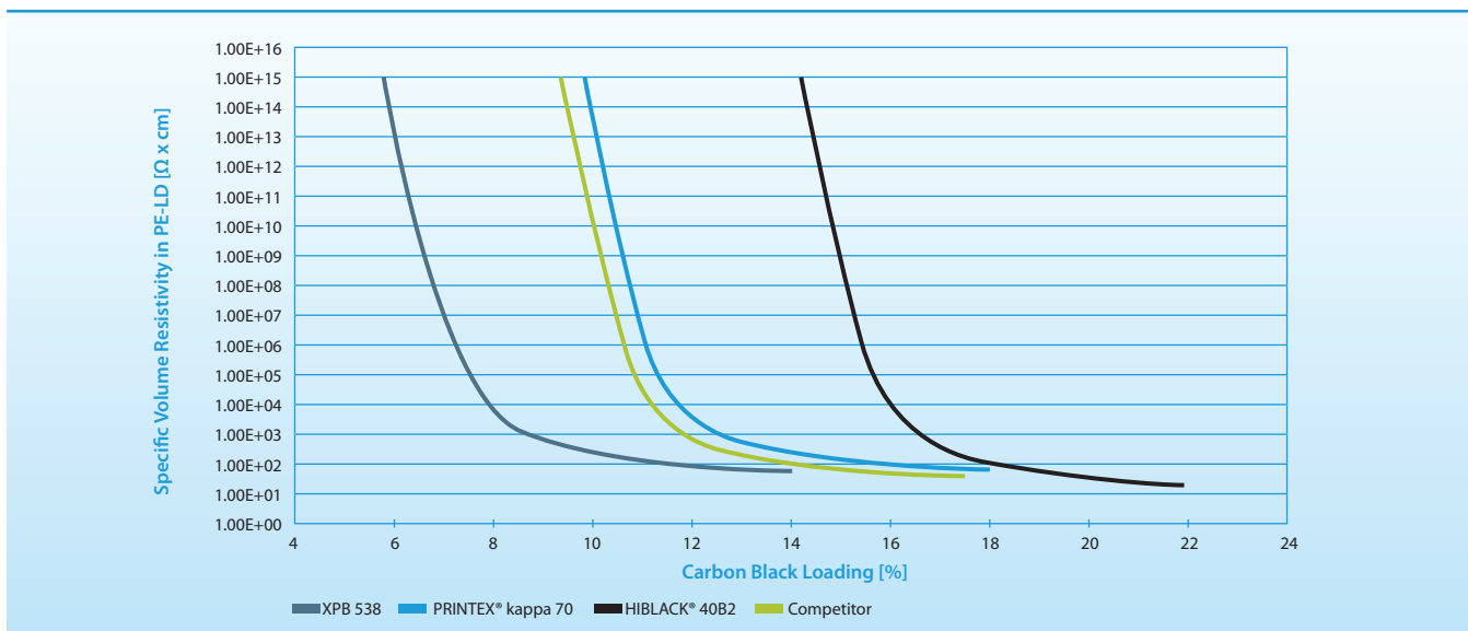
Figure 3 The Influence of the Specialty Carbon Black Content on the electrical Resistivity of Polymers
